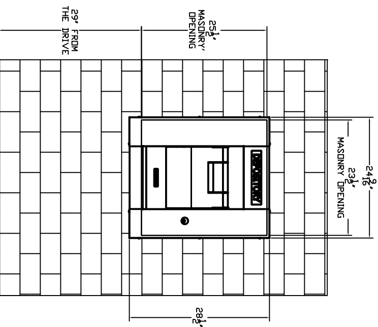
MASONRY DETAIL
